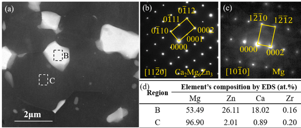
Fig. 9. (a) The HADDF-TEM image of the ZK416 alloy and (b, c) the corresponding SAED patterns of the distinct regions marked as B and C in (a), (d) the EDS chemical compositions of the distinct regions B and C in (a).
