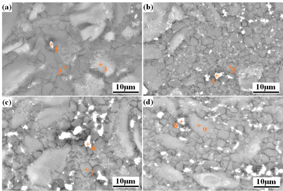
Fig. 3. The SEM images of the as-extruded captured from the plane normal to ED (a) ZK41, (b) ZK413, (c) ZK416 and (d) ZK419 alloy.
