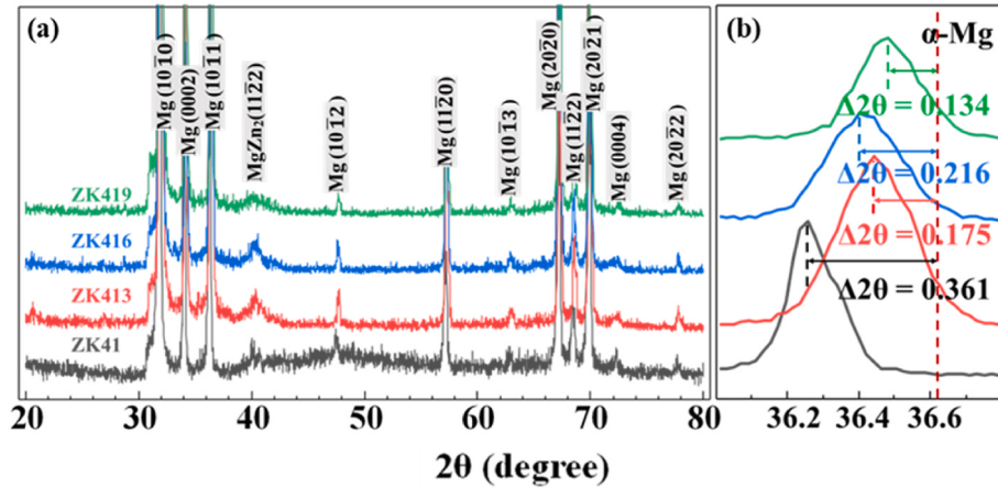
Fig. 8. (a) XRD patterns of the as-extruded Mg-4Zn-0.6Zr-xCa (x = 0, 0.3, 0.6, 0.9 wt%) alloys and (b) The offset of the \alpha -Mg peak near 2θ = 36.60 of the as-extruded Mg-4Zn-0.6Zr-xCa (x = 0, 0.3, 0.6, 0.9 wt%) alloys.
